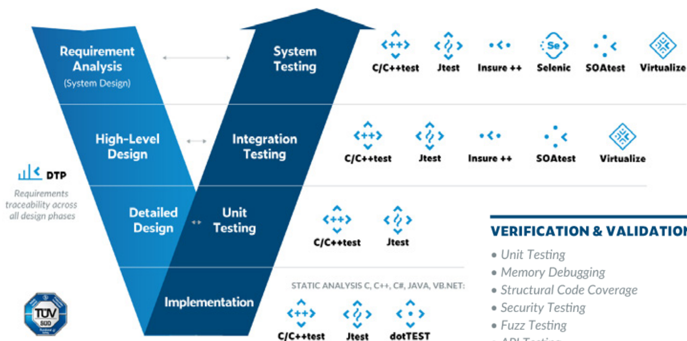
Figure 5: V-model for software development.
